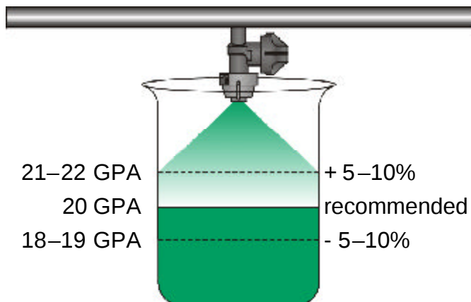
Figure 12b. If measured rate is between 5 percent and 10 percent of recommended GPA, try adjusting pressure. Lower pressure to deliver less spray, or raise pressure to deliver more. Recheck output.
