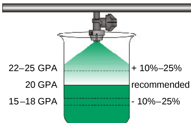
Figure 12c. If measured rate varies by more than 10 percent, but less than 25 percent, adjust speed. Slower speed delivers more spray, and faster speed delivers less. Measure speed under field conditions, insert the new speed into the equation to determine GPA, and recheck output.
