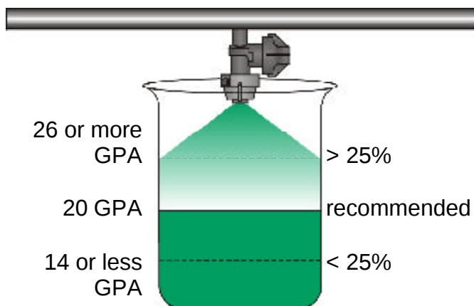
Figure 12d. If measured rate varies by more than 25 percent, change nozzles and repeat the pre-calibration and calibration processes.
