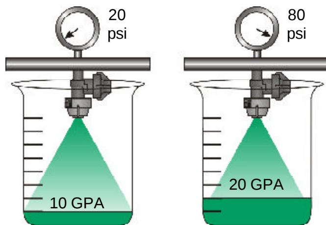
Figure 5. Pressure must be increased four times to double sprayer output.
